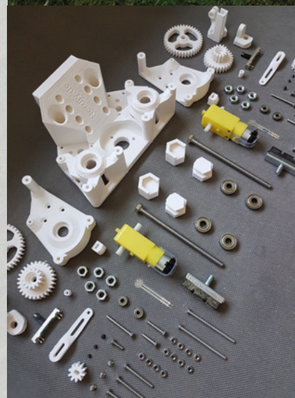
Left ◀ Almost every part of WinDIY is 3D printed from scratch
