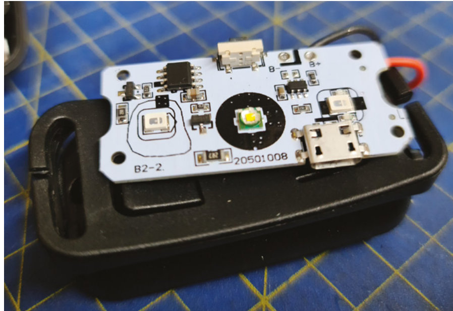
Above ♦ You can clearly see that this lamp has a tiny PCB-mounted switch at the top that would be crushed into oblivion by chunky welding glove fingers. Next to it, on the right, are the main battery connections. These are the areas that you need to solder onto extension wires onto
