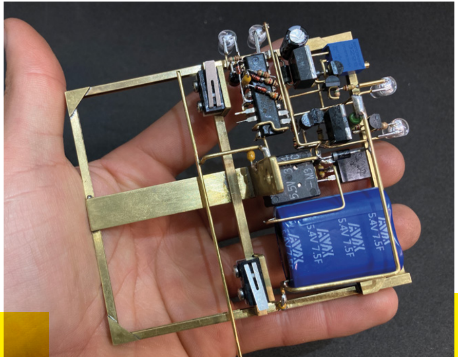
Above ↑ The completed solar logic
